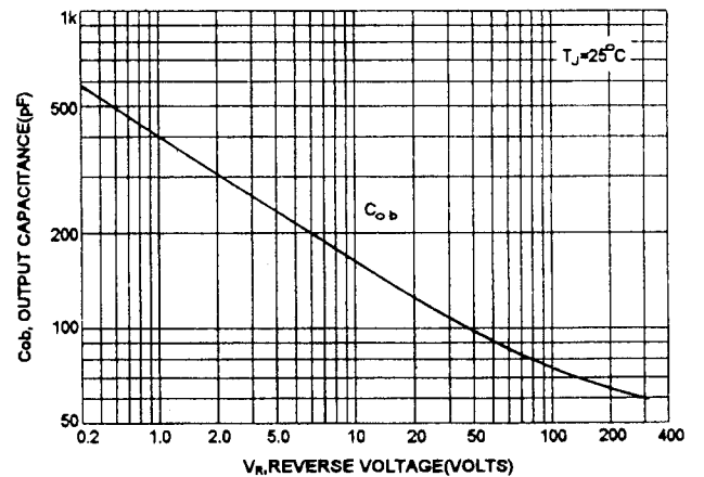
OUTPUT CAPACITANCES
